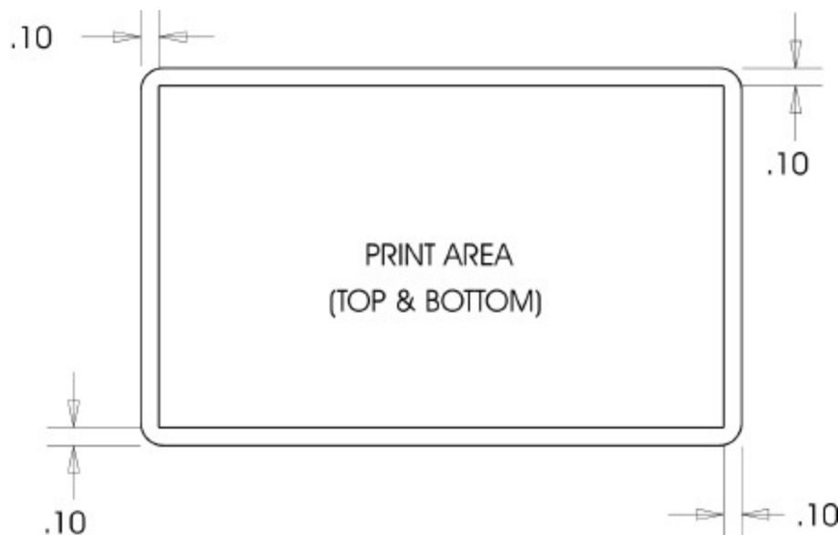
Rear Monochrome Graphics Printer
