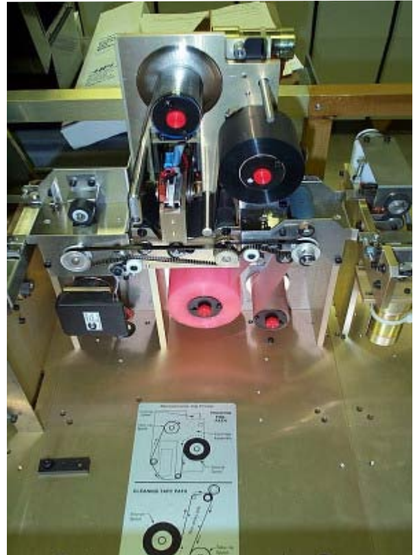
Front Monochrome Graphics Printer
